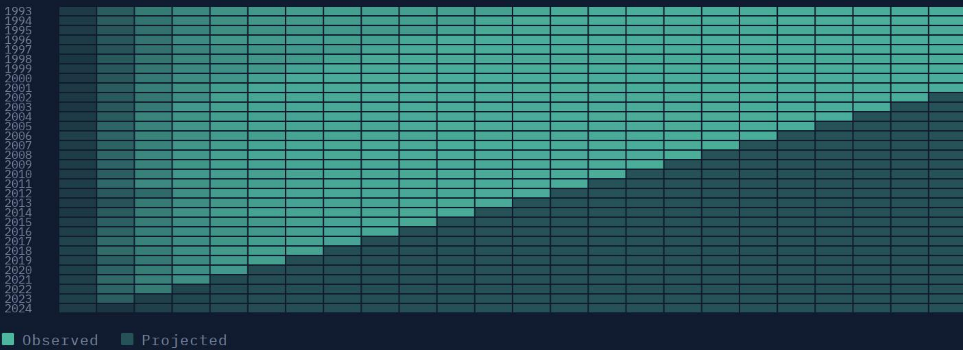
Fig. 1.2 % of ultimate by accident year
