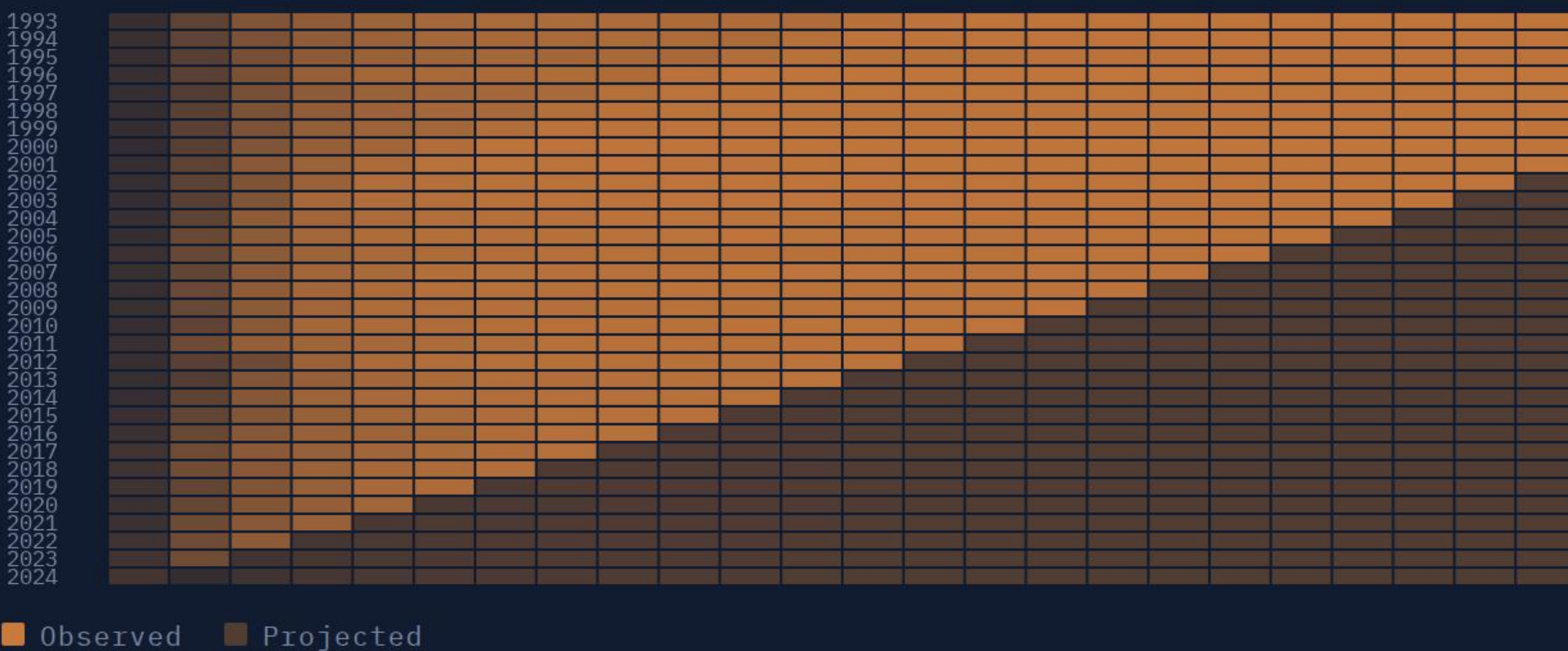
Fig. 3.2 % of ultimate by accident year
